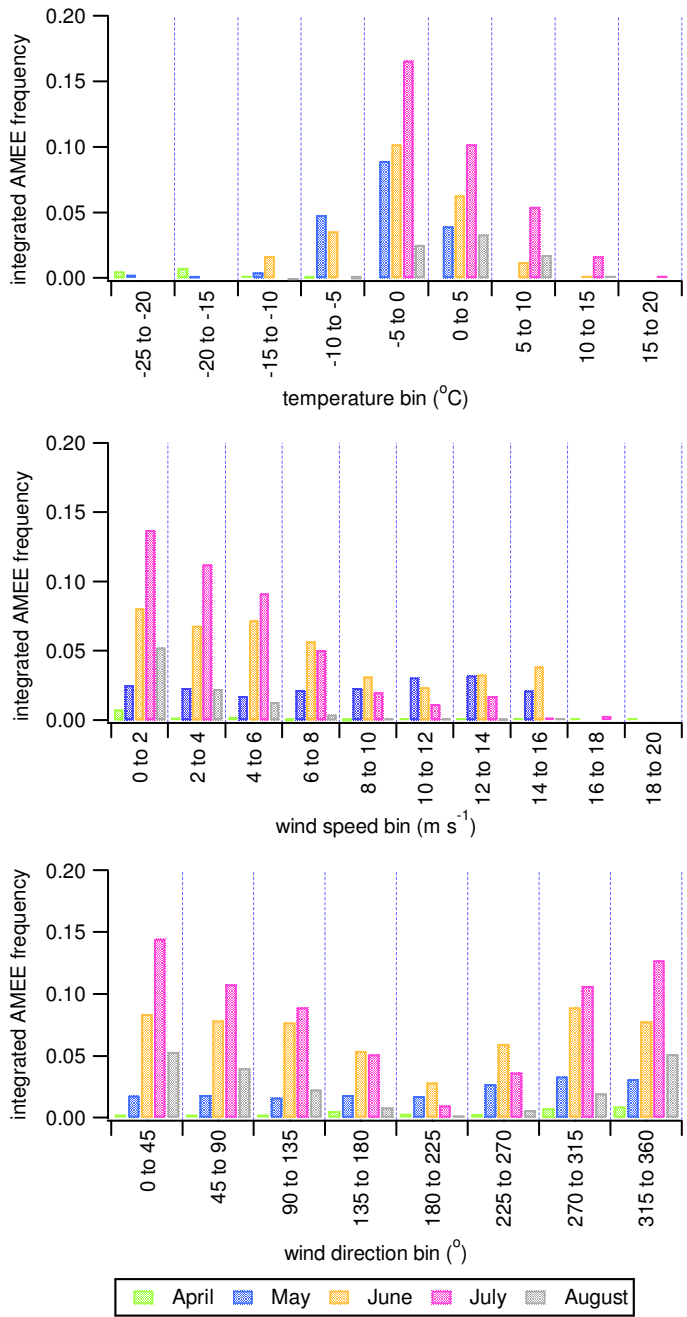
Figure 4: Integrated AMEE frequency as a function of temperature, wind speed, wind direction and month for Alert data 1995-2007. Note the change in scale from Figures 2 and 3.
