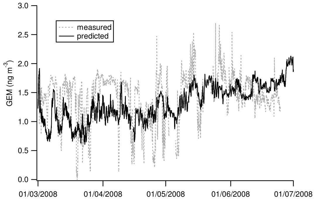
Figure 5: Comparison of measured GEM concentrations at Alert for March-June 2008 with those predicted based on a multiple linear regression fit of 1995-2007 GEM concentrations to local temperature and Julian day.
